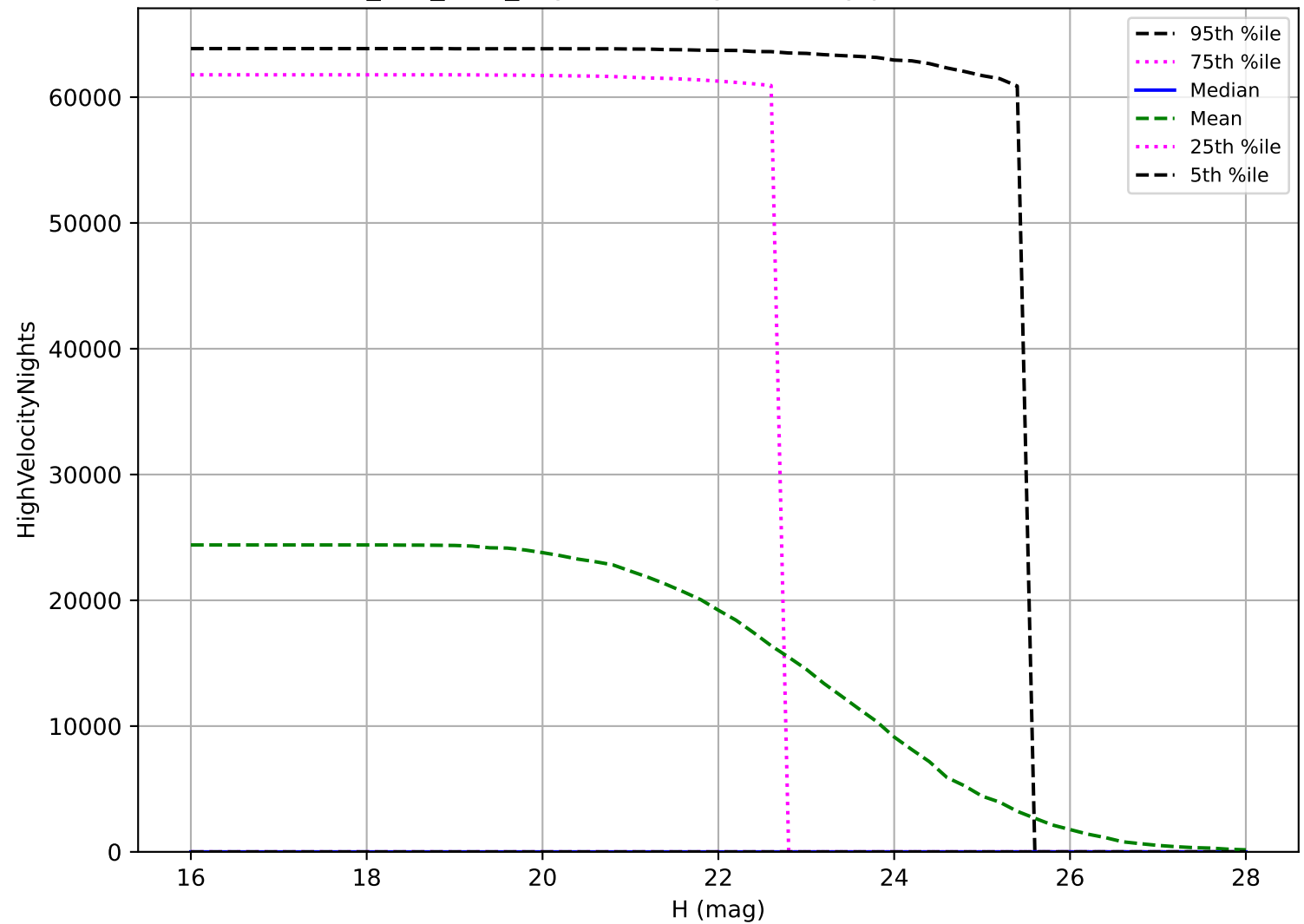
smc_lmc_v3.3_10yrs: PHA High velocity pair detection loss
