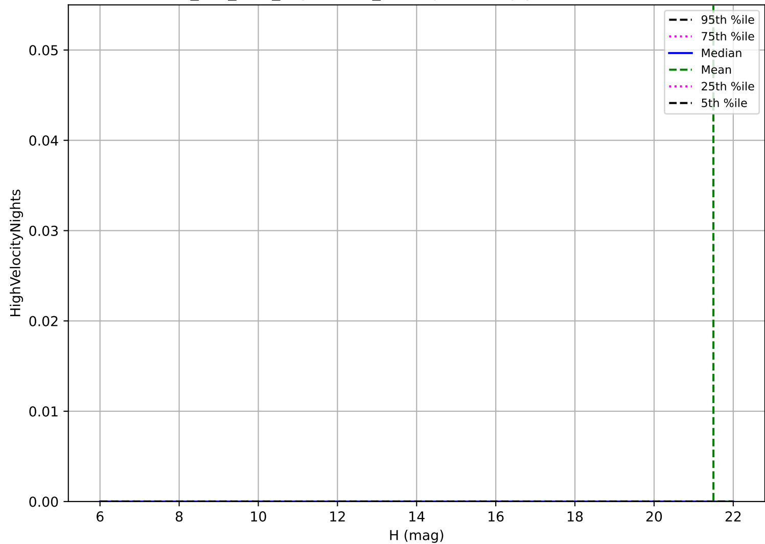
smc_lmc_v3.3_10yrs: OCC_r20 High velocity pair detection loss
