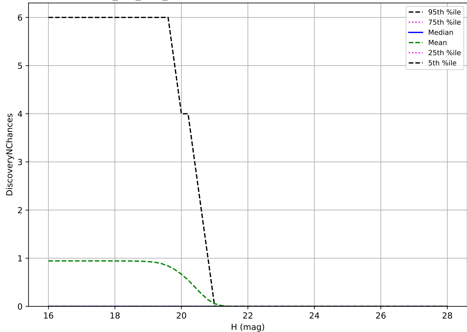
smc_lmc_v3.3_10yrs: Vatira 3 pairs in 15 nights detection loss
