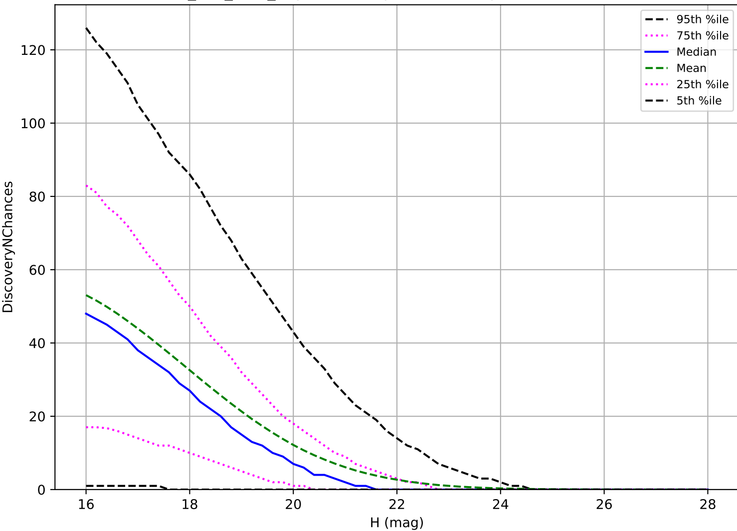
smc_lmc_v3.3_10yrs: PHA 3 pairs in 15 nights detection loss
