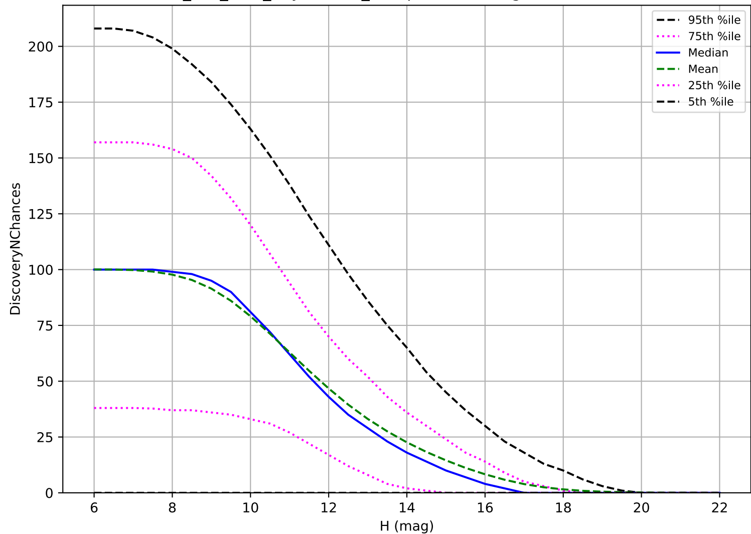
smc_lmc_v3.3_10yrs: OCC_r5 3 pairs in 15 nights detection loss
