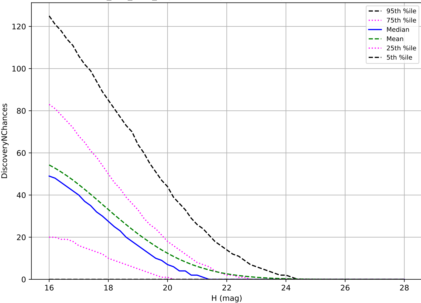
smc_lmc_v3.3_10yrs: NEO 3 pairs in 15 nights detection loss
