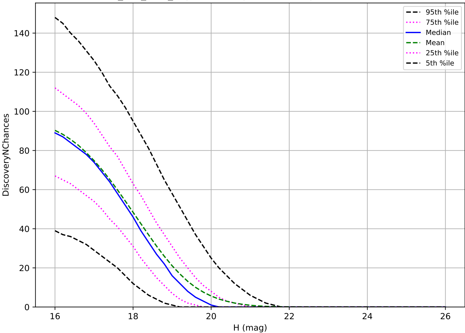
smc_lmc_v3.3_10yrs: MBA 3 pairs in 15 nights detection loss
