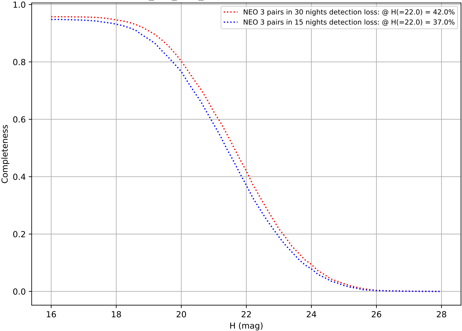
smc_lmc_v3.3_10yrs: DifferentialCompleteness
