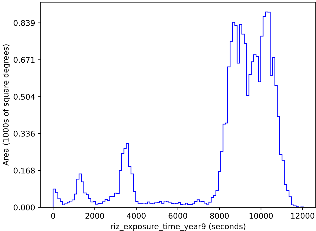
smc_lmc_v3.3_10yrs gri band non-DD: riz_exposure_time_year9
