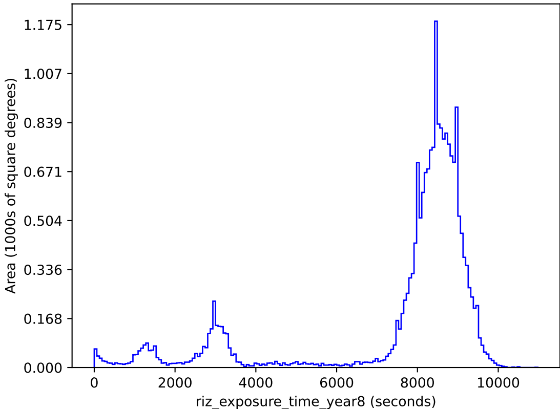
smc_lmc_v3.3_10yrs gri band non-DD: riz_exposure_time_year8
