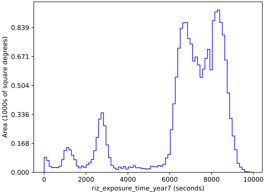
smc_lmc_v3.3_10yrs gri band non-DD: riz_exposure_time_year7
