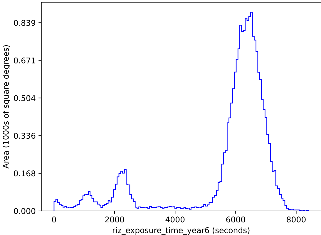
smc_lmc_v3.3_10yrs gri band non-DD: riz_exposure_time_year6
