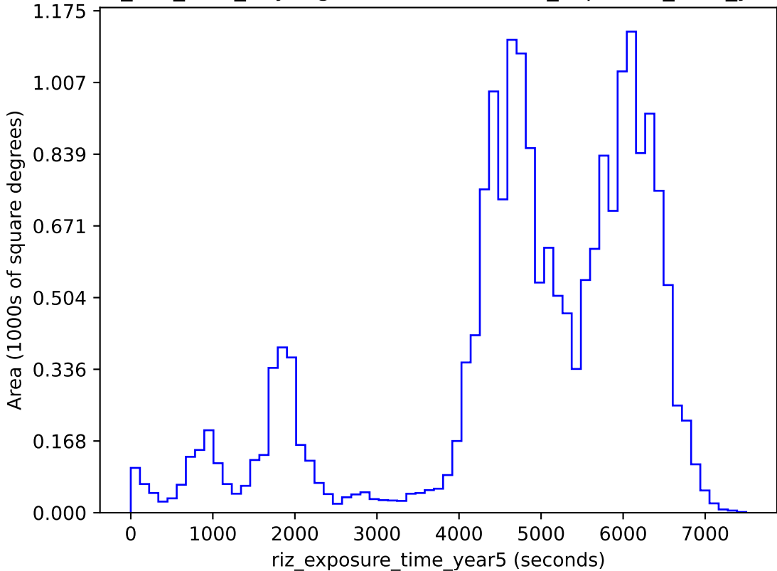
smc_lmc_v3.3_10yrs gri band non-DD: riz_exposure_time_year5
