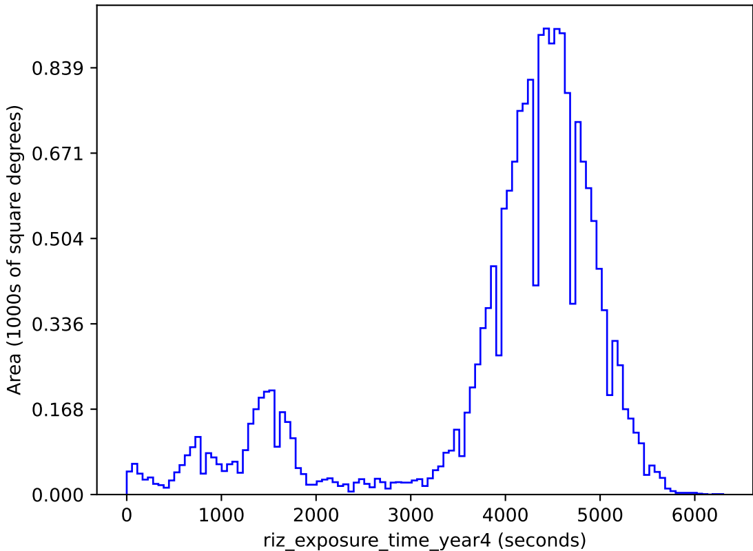
smc_lmc_v3.3_10yrs gri band non-DD: riz_exposure_time_year4
