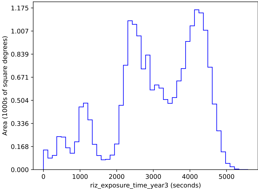
smc_lmc_v3.3_10yrs gri band non-DD: riz_exposure_time_year3
