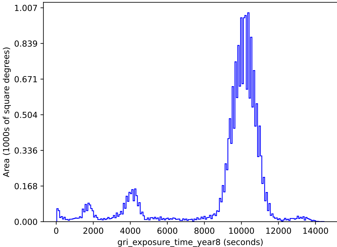
smc_lmc_v3.3_10yrs gri band non-DD: gri_exposure_time_year8
