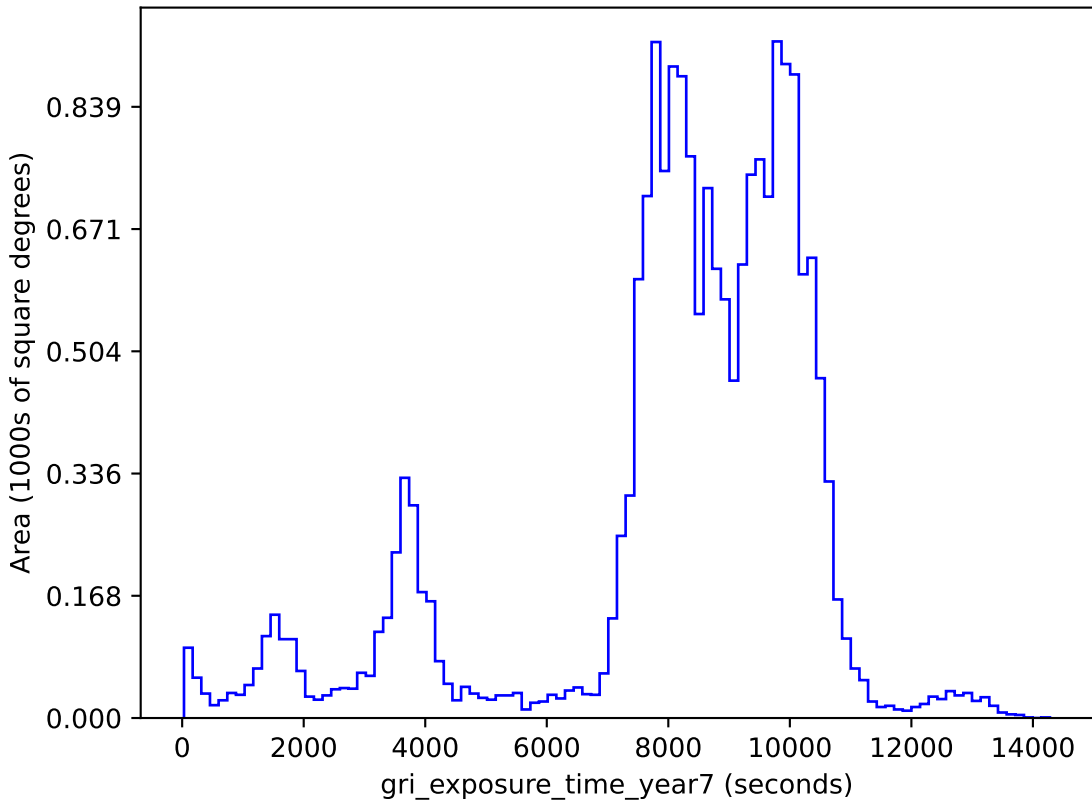
smc_lmc_v3.3_10yrs gri band non-DD: gri_exposure_time_year7
