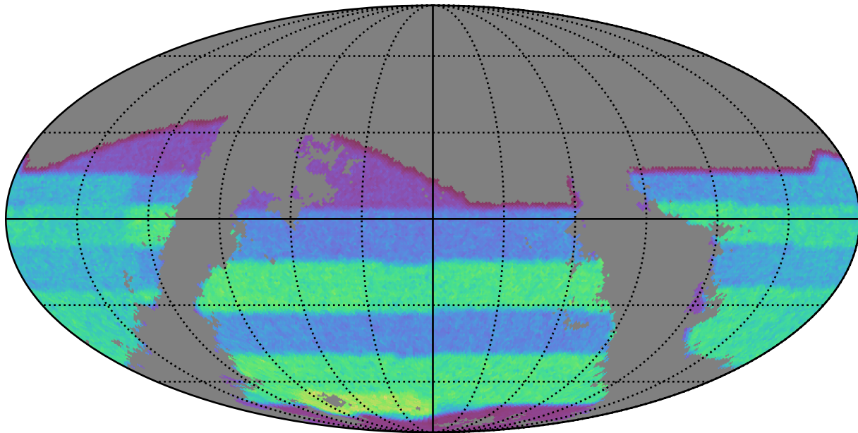
smc_lmc_v3.3_10yrs gri band non-DD: gri_exposure_time_year3
