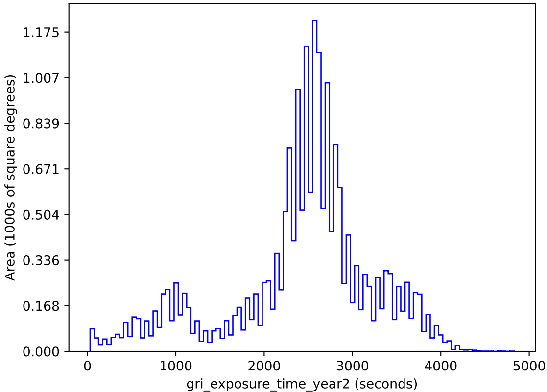
smc_lmc_v3.3_10yrs gri band non-DD: gri_exposure_time_year2
