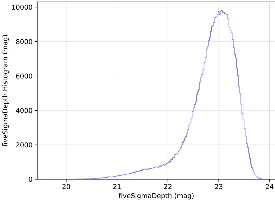
smc_lmc_v3.3_10yrs z: fiveSigmaDepth Histogram
