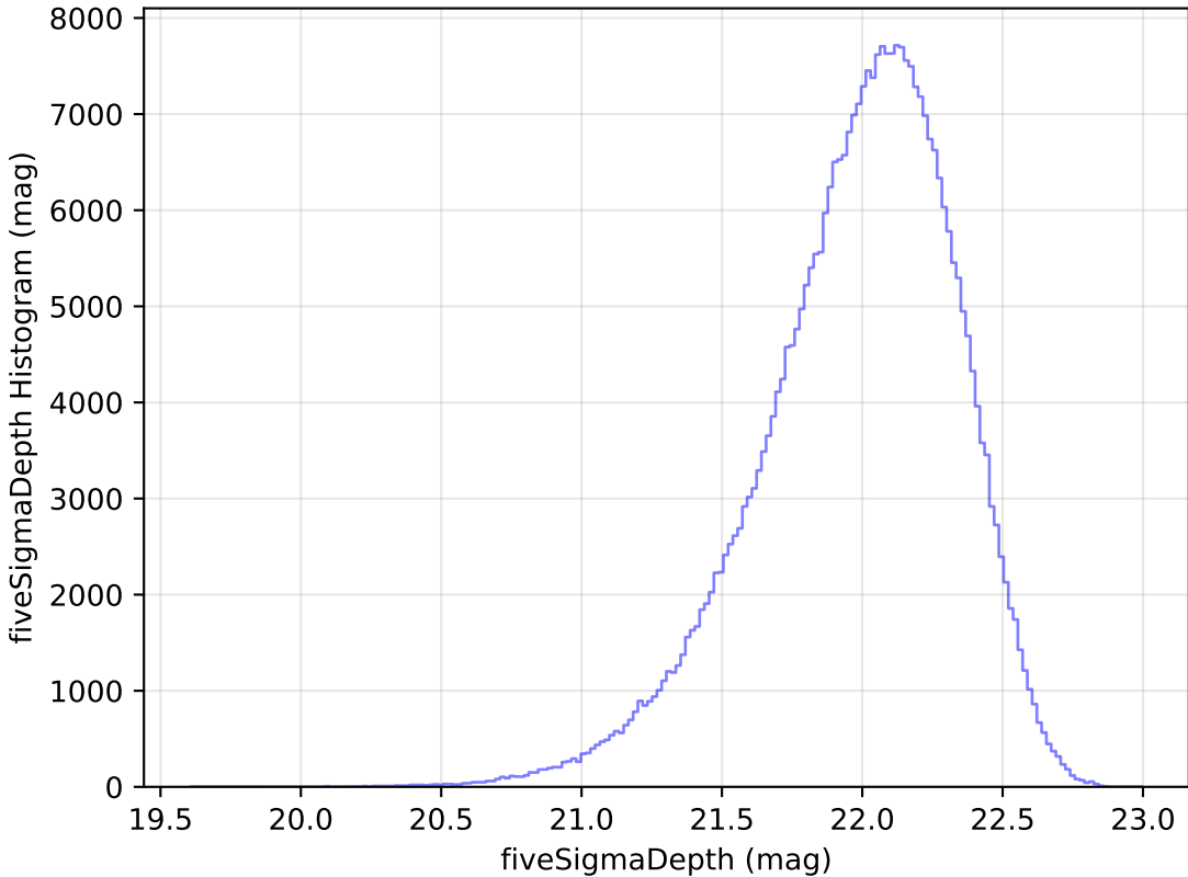
smc_lmc_v3.3_10yrs y: fiveSigmaDepth Histogram
