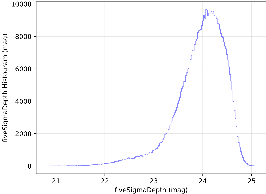
smc_lmc_v3.3_10yrs r: fiveSigmaDepth Histogram
