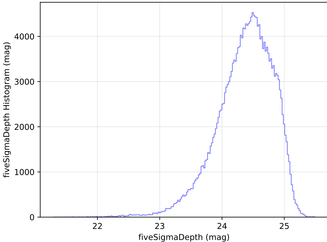
smc_lmc_v3.3_10yrs g: fiveSigmaDepth Histogram
