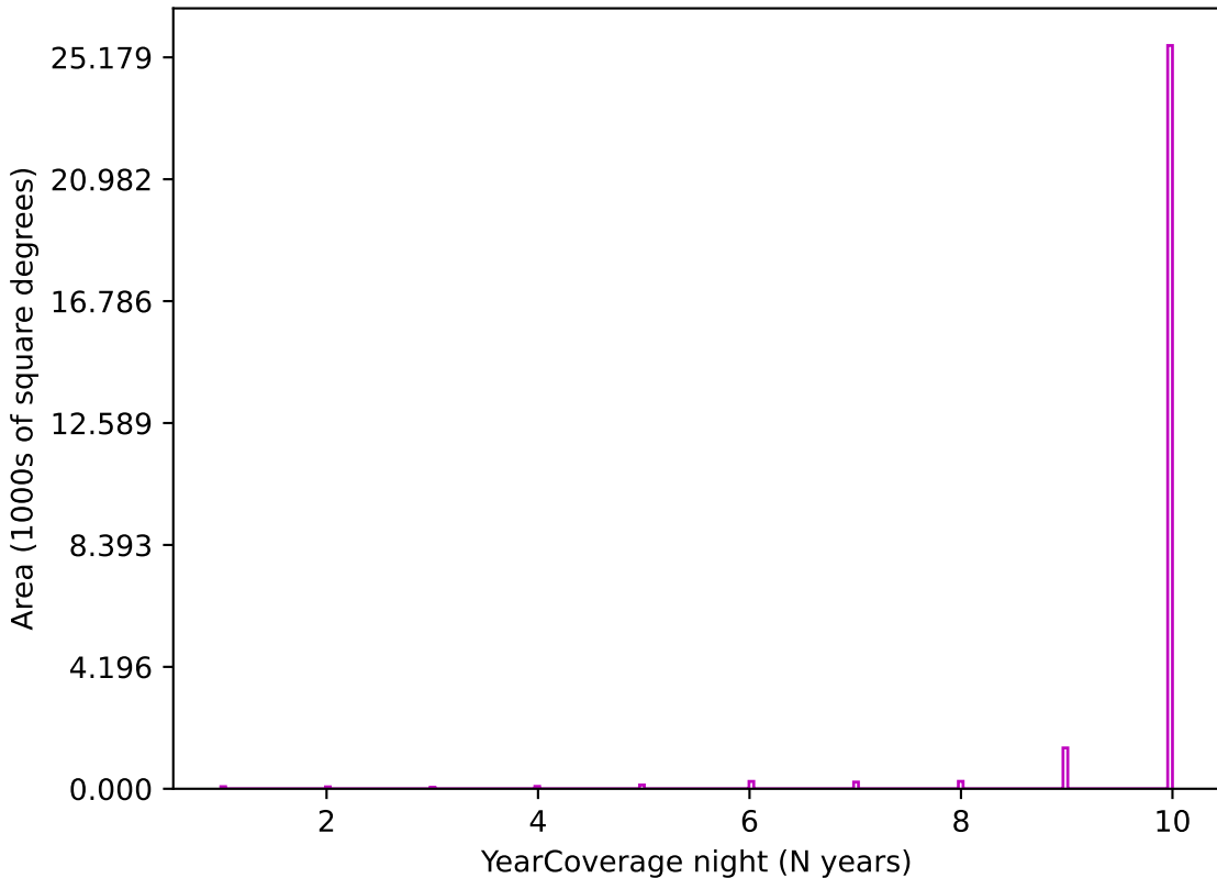
smc_lmc_v3.3_10yrs z band: YearCoverage night
