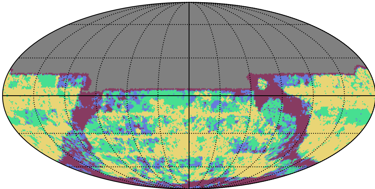
smc_lmc_v3.3_10yrs u band: YearCoverage night
