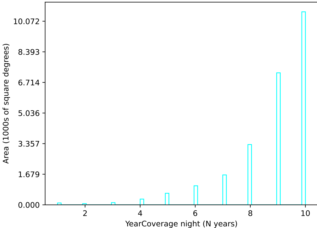
smc_lmc_v3.3_10yrs u band: YearCoverage night
