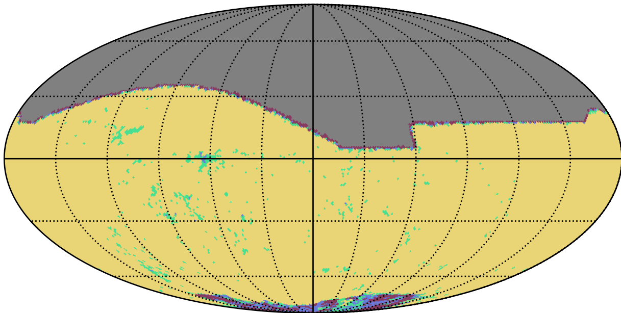
smc_lmc_v3.3_10yrs i band: YearCoverage night
