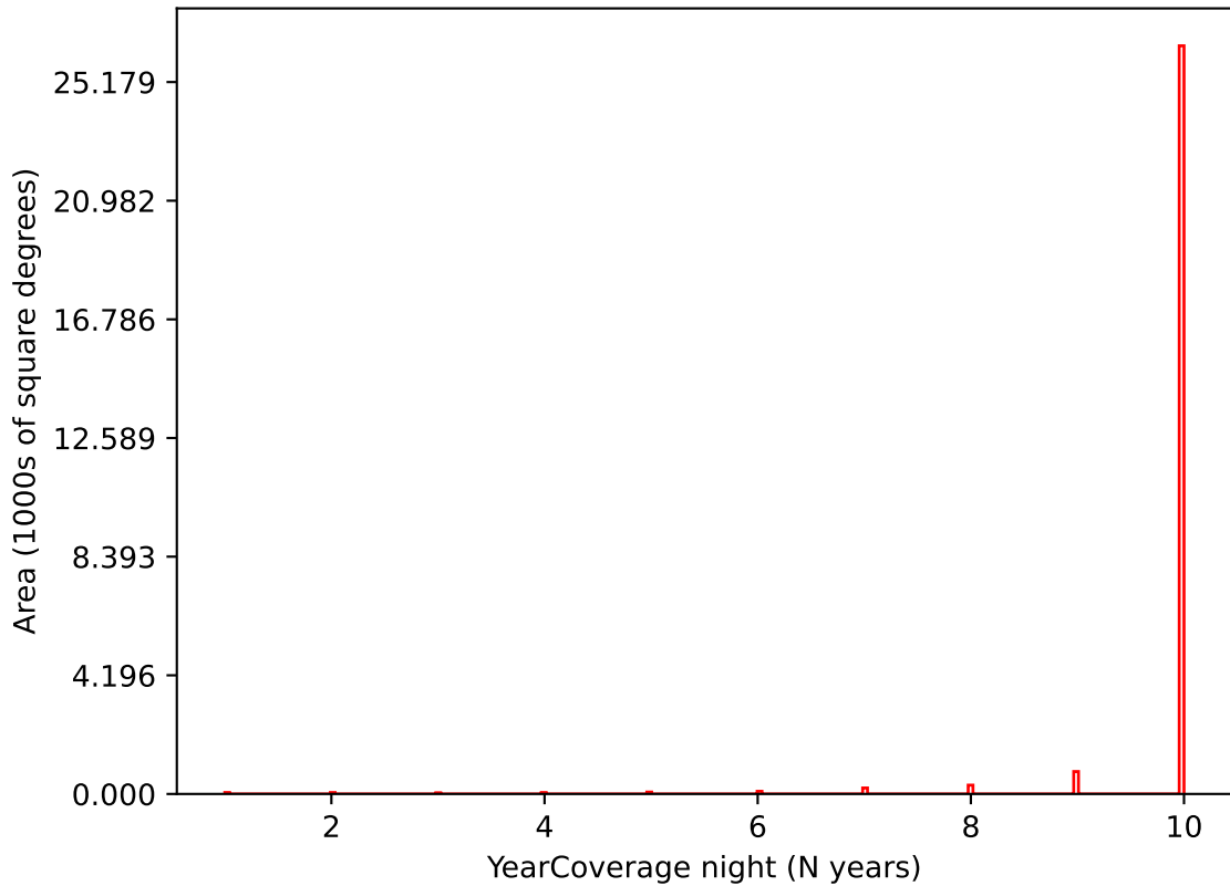
smc_lmc_v3.3_10yrs i band: YearCoverage night
