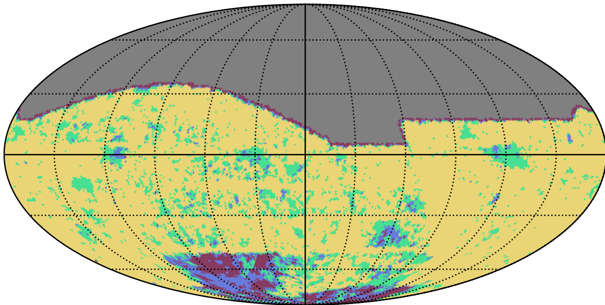
smc_lmc_v3.3_10yrs g band: YearCoverage night
