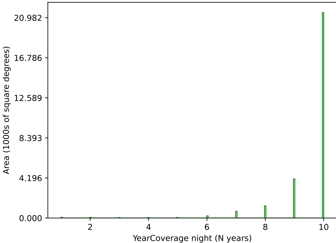
smc_lmc_v3.3_10yrs g band: YearCoverage night
