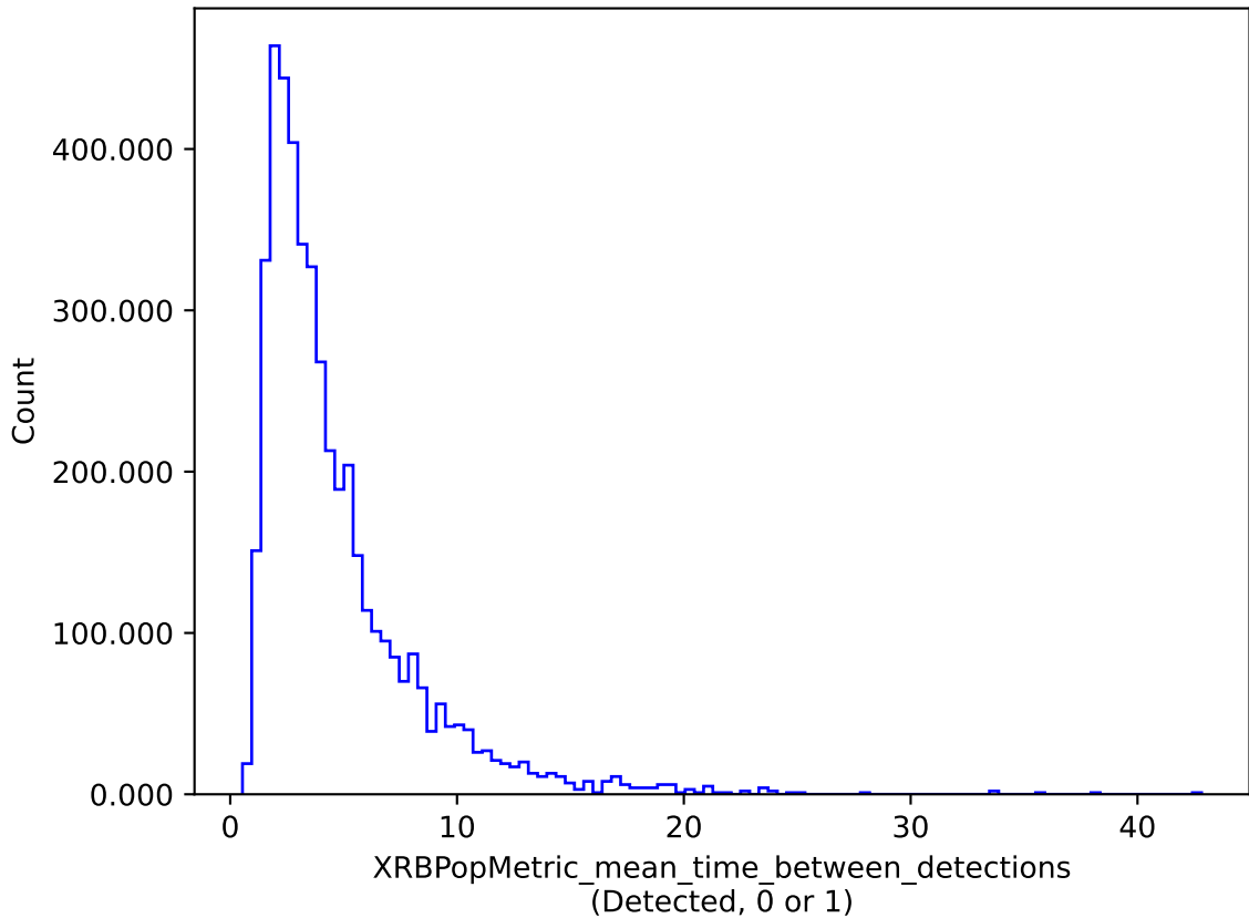
smc_Imc_v3.3_10yrs : XRBPoMetric_mean_time_between_detections
