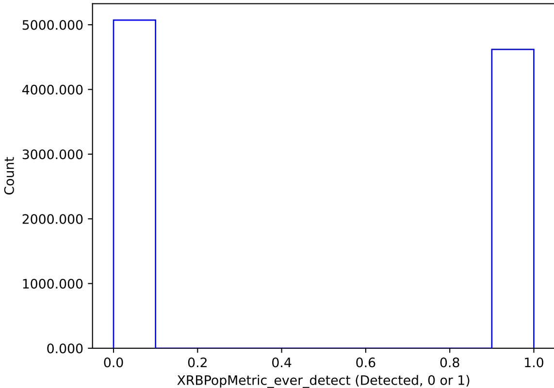
smc_lmc_v3.3_10yrs : XRBPopMetric_ever_detect
