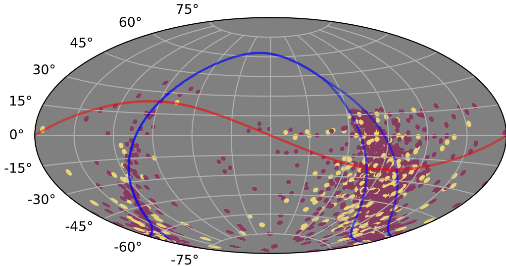
smc_lmc_v3.3_10yrs : XRBPoPmetric_early_detect
