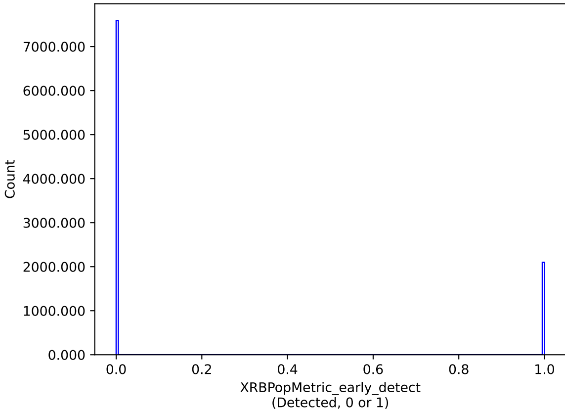
smc_lmc_v3.3_10yrs : XRBPoMetric_early_detect
