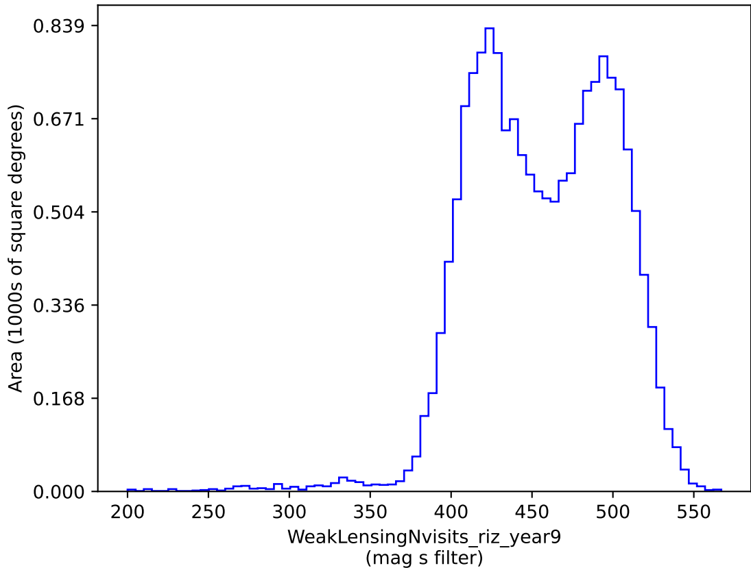
smc_Imc_v3.3_10yrs gri band non-DD: WeakLensingNvisits_riz_year9
