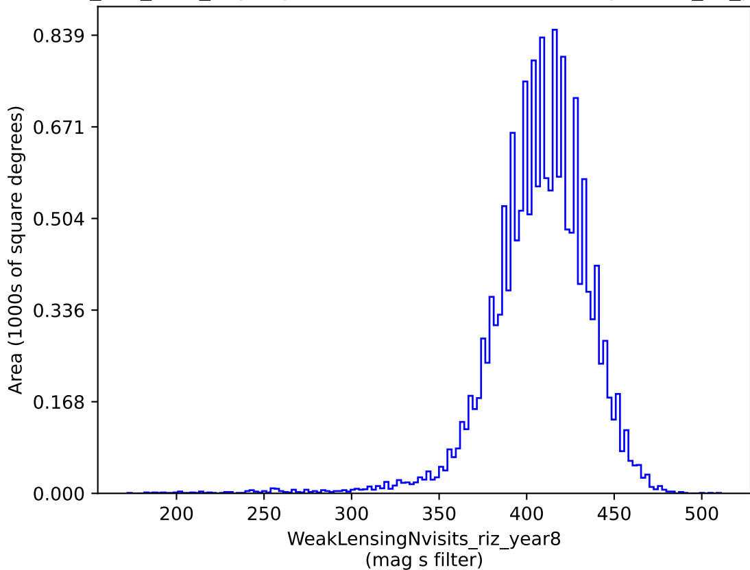
smc_Imc_v3.3_10yrs gri band non-DD: WeakLensingNvisits_riz_year8
