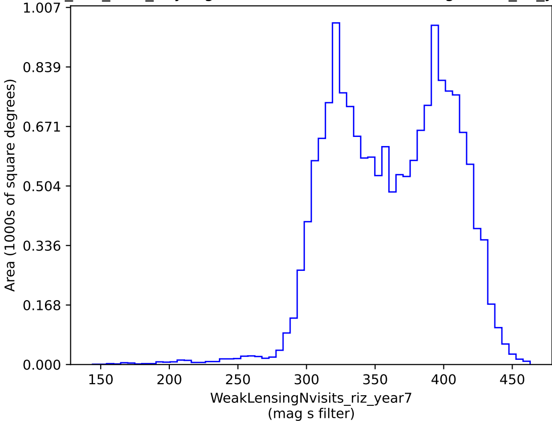
smc_Imc_v3.3_10yrs gri band non-DD: WeakLensingNvisits_riz_year7
