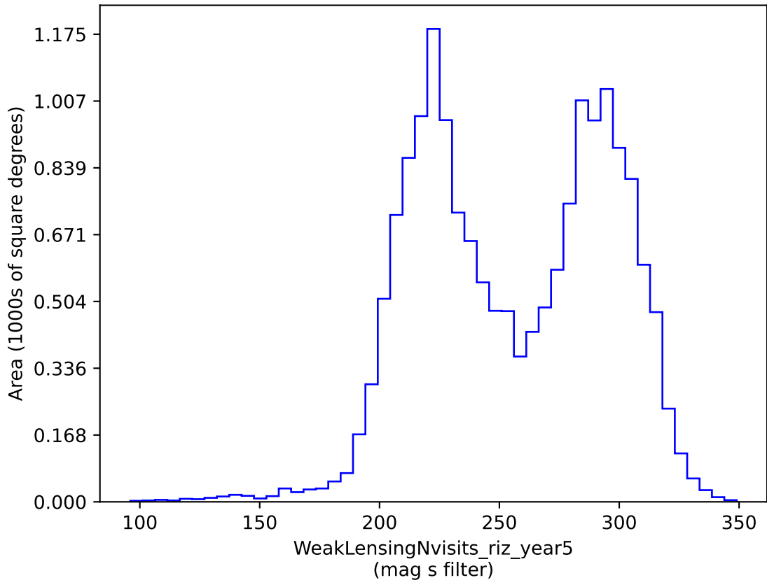
smc_Imc_v3.3_10yrs gri band non-DD: WeakLensingNvisits_riz_year5
