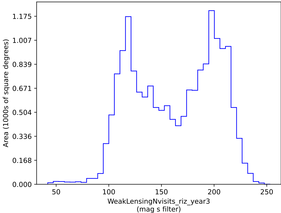
smc_Imc_v3.3_10yrs gri band non-DD: WeakLensingNvisits_riz_year3
