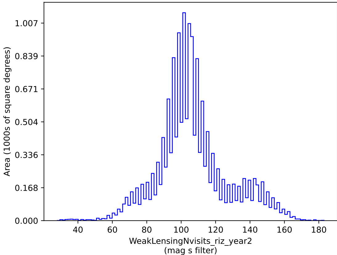
smc_Imc_v3.3_10yrs gri band non-DD: WeakLensingNvisits_riz_year2
