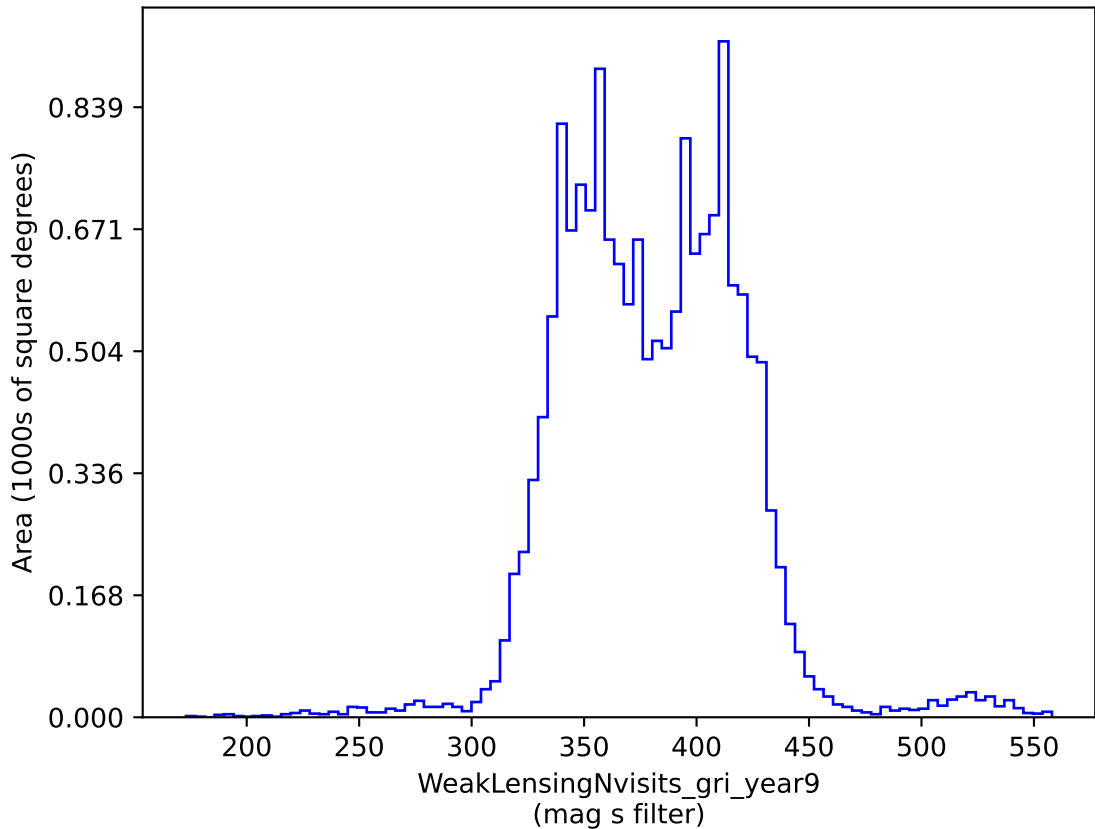
smc_Imc_v3.3_10yrs gri band non-DD: WeakLensingNvisits_gri_year9
