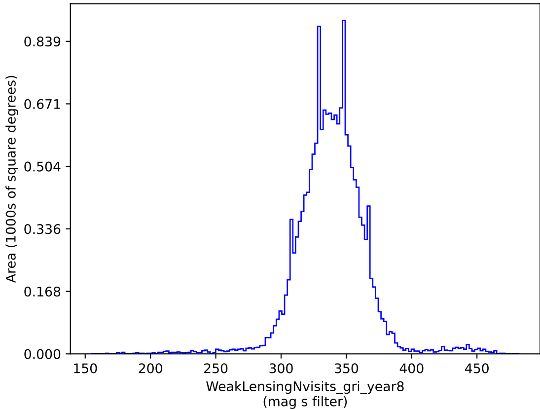
smc_lmc_v3.3_10yrs gri band non-DD: WeakLensingNvisits_gri_year8
