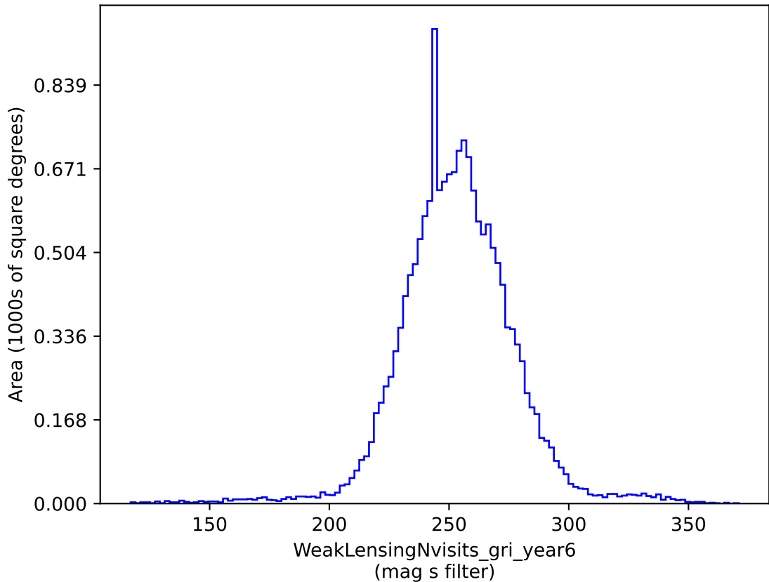
smc_lmc_v3.3_10yrs gri band non-DD: WeakLensingNvisits_gri_year6
