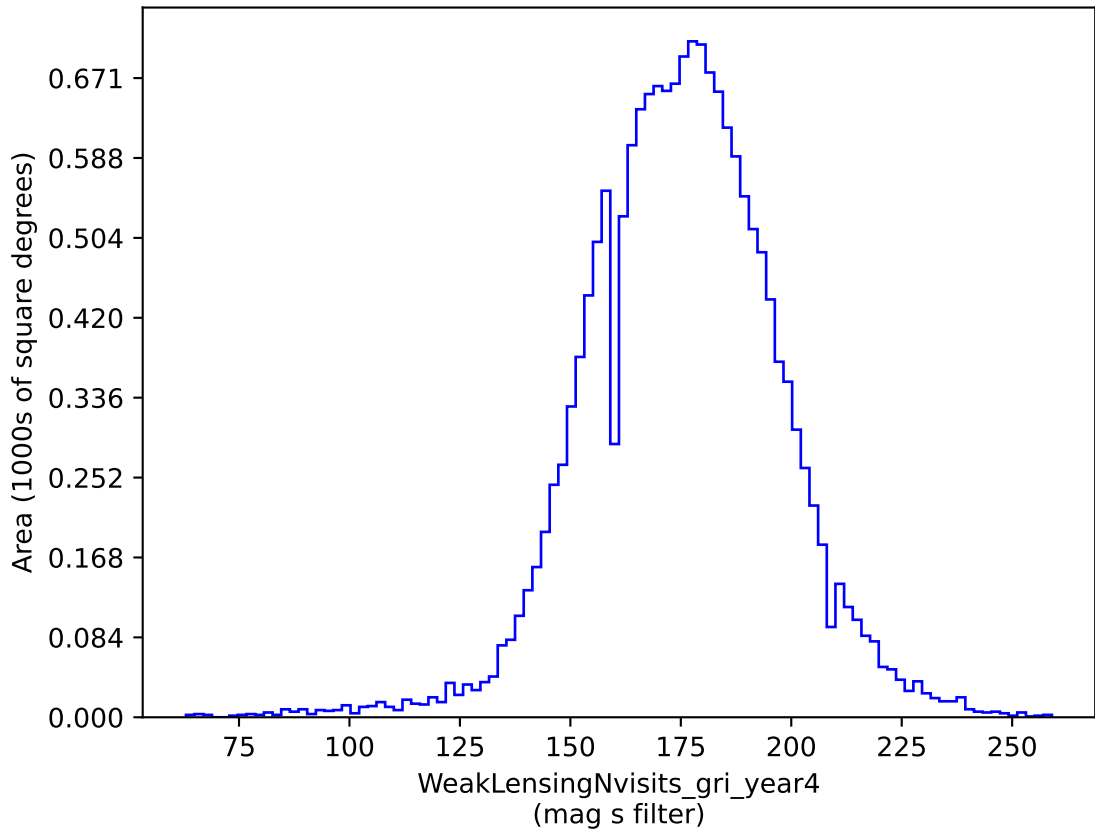
smc_lmc_v3.3_10yrs gri band non-DD: WeakLensingNvisits_gri_year4
