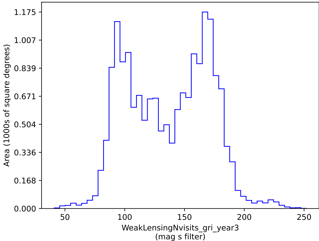
smc_lmc_v3.3_10yrs gri band non-DD: WeakLensingNvisits_gri_year3
