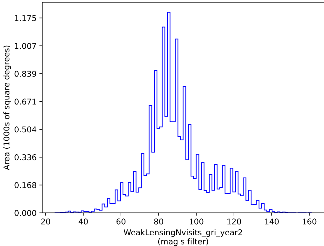
smc_lmc_v3.3_10yrs gri band non-DD: WeakLensingNvisits_gri_year2
