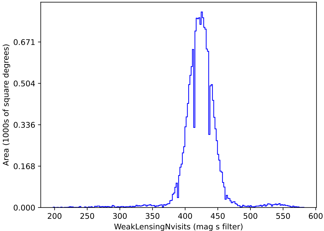
smc_lmc_v3.3_10yrs gri band non-DD: WeakLensingNvisits
