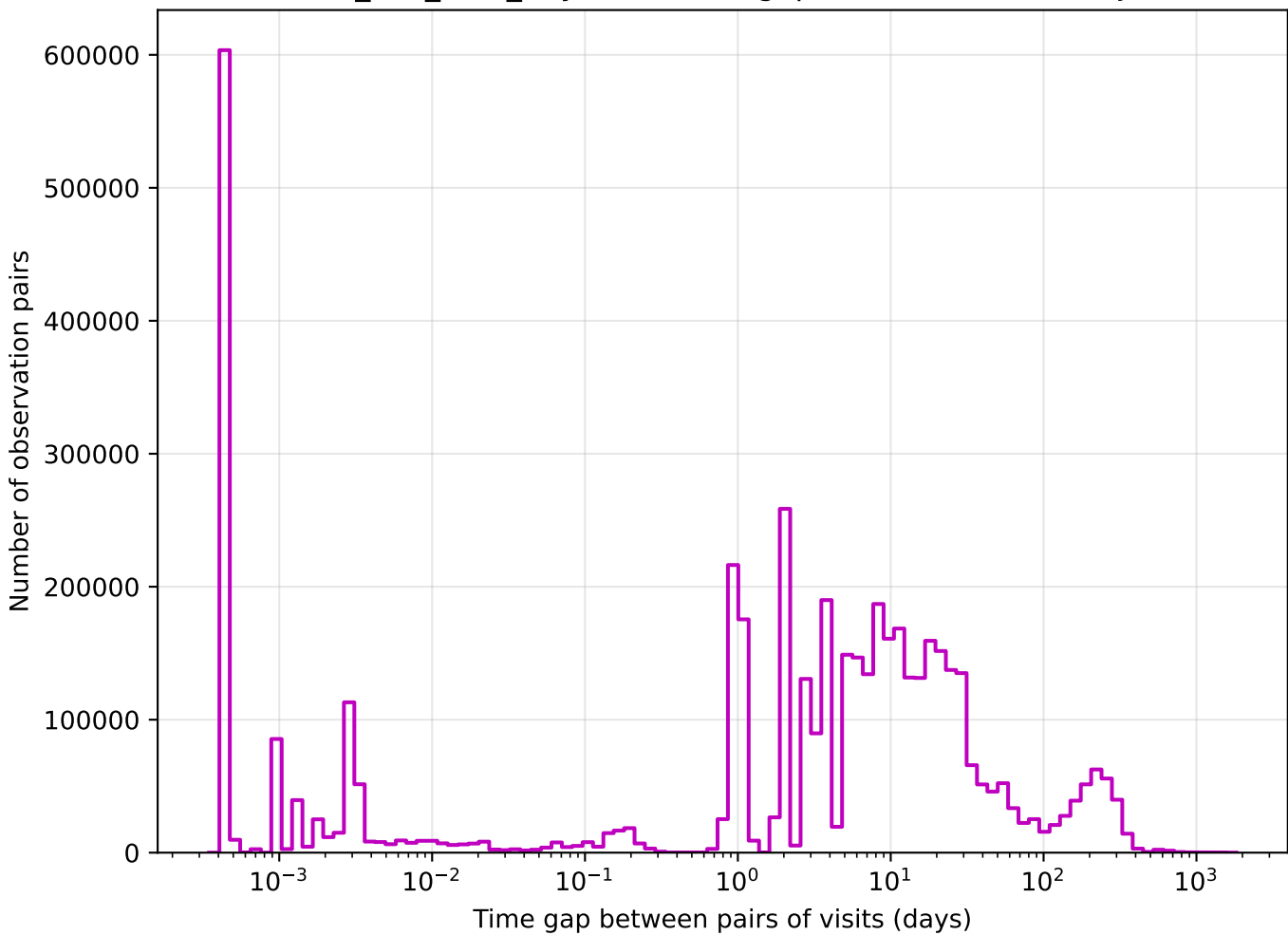
smc_lmc_v3.3_10yrs z band: Tgaps observationStartMJD
