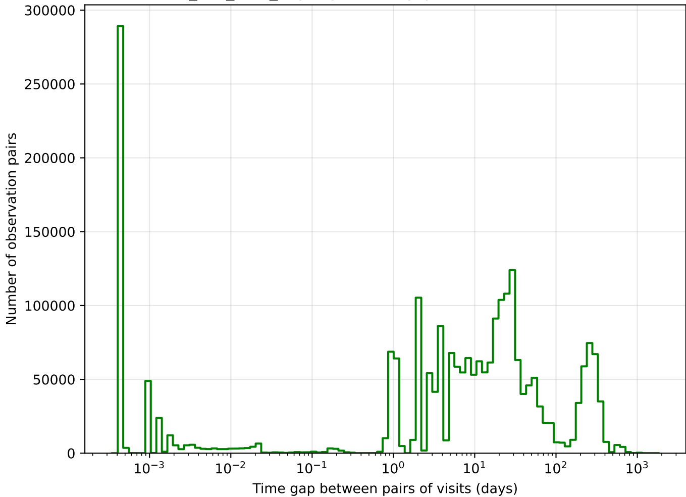
smc_lmc_v3.3_10yrs g band: Tgaps observationStartMJD
