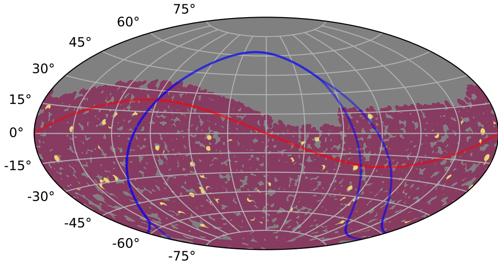
smc_lmc_v3.3_10yrs : TDEsPopMetric_some_color_pu
